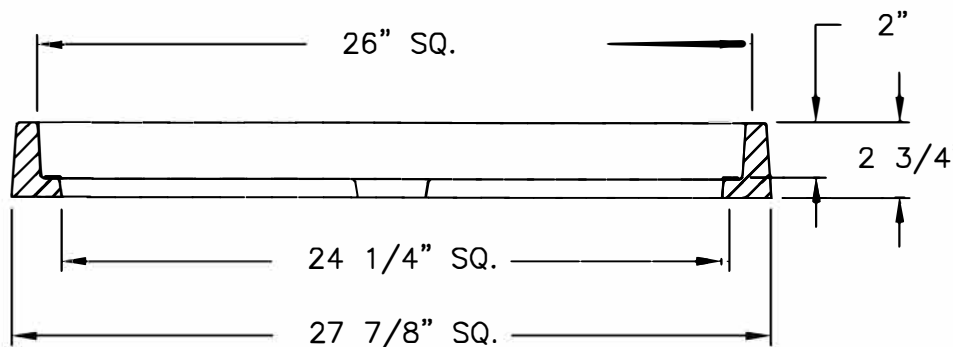
FRAME SECTION
